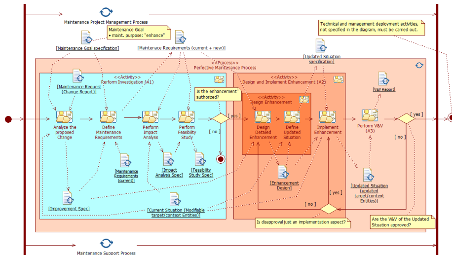
Fig. 4. Maintenance Process Specification for the Perfective Maintenance Strategy of the family considering the behavioral and functional perspectives.
