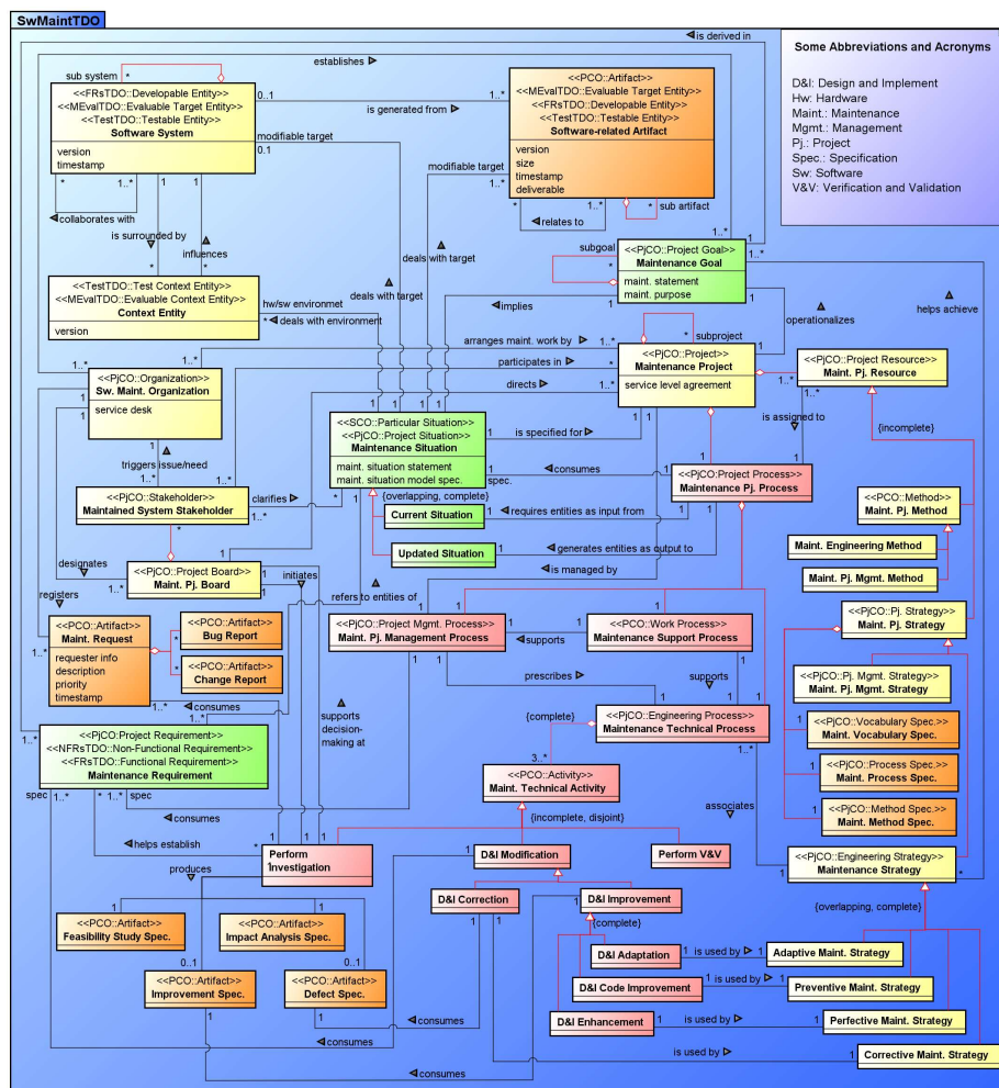
Fig. 2. Excerpt of SwMaintTDO v1.0: Top-Domain Ontology for Software Maintenance.
