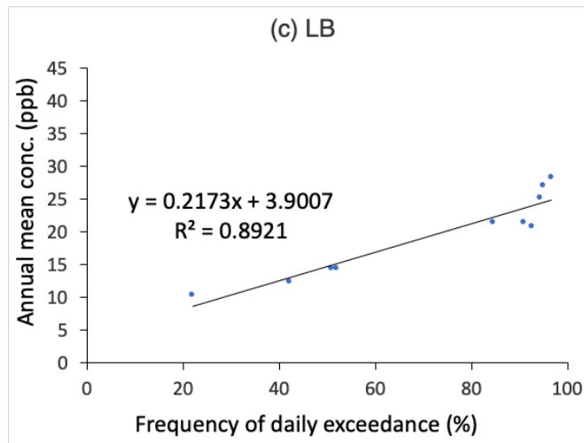
Figure A.1: Scatter plot of annual mean NO 2 concentration vs frequency of daily mean NO 2 concentration exceeding the WHO guideline level (13 ppb) at: a) CEN, b) COR and c) LB. The linear fit is included.
