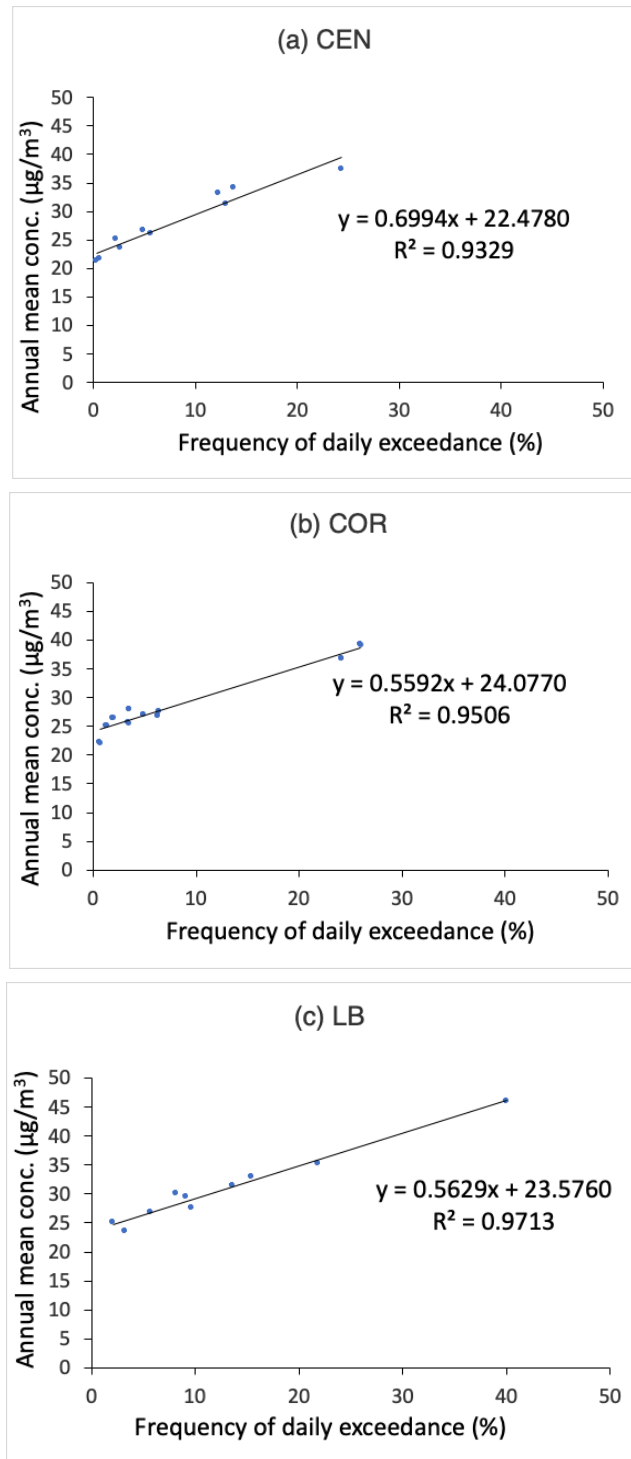
Figure A.2: Scatter plot of annual mean \text{PM}_{10} concentration vs frequency of daily mean \text{PM}_{10} concentration exceeding the WHO guideline level ( 45 \mu\text{g m}^{-3} ) at: a) CEN, b) COR
