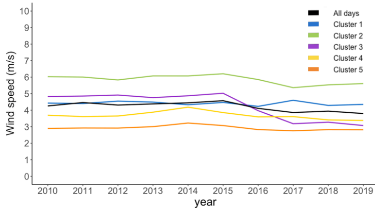
Figure 3: Interannual variation of mean wind speed measured at the AEP meteorological station, considering all data (black) and grouping days by wind cluster (color code).
