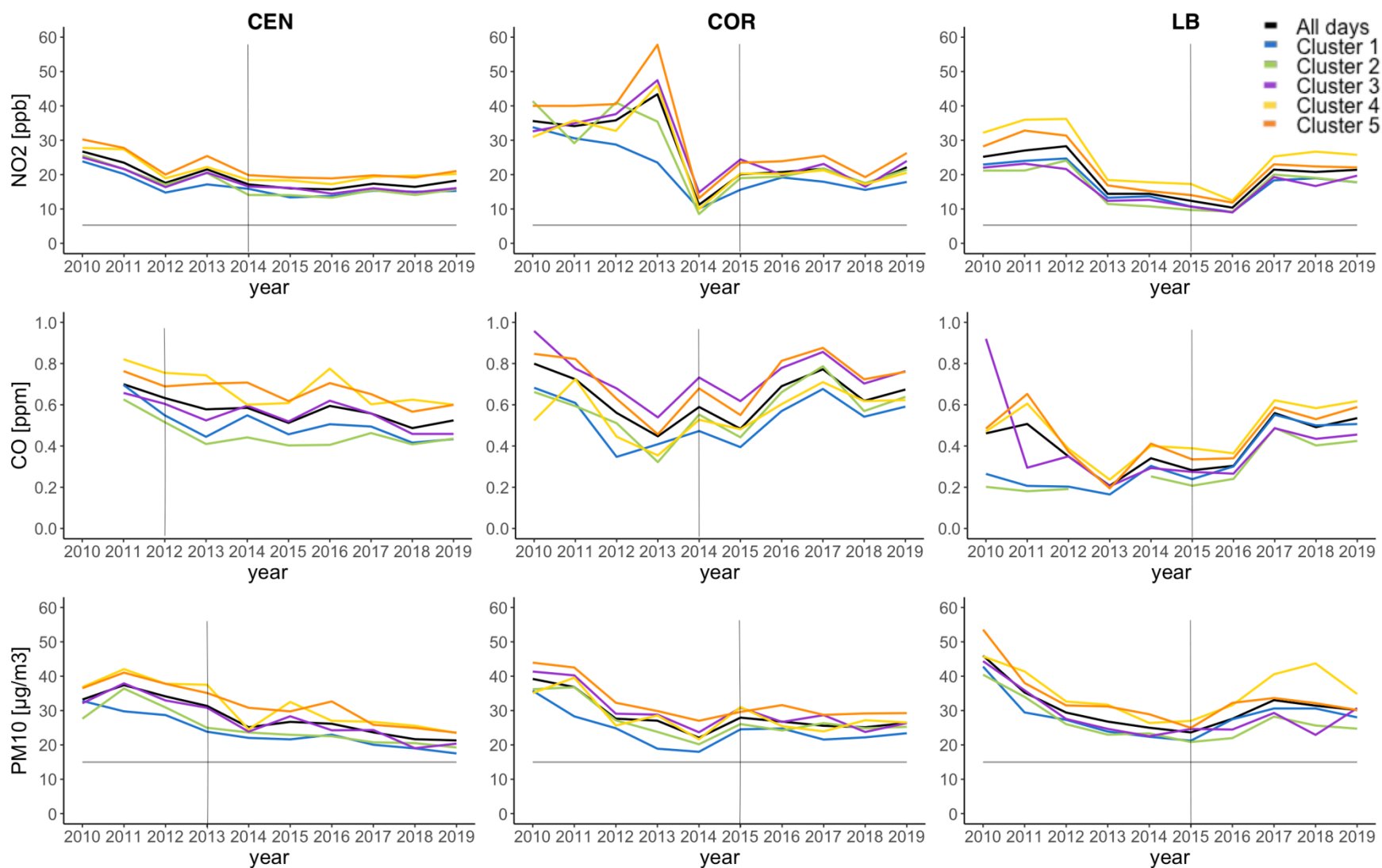
Figure 2: Interannual variation of air pollutant concentrations at each monitoring site (CEN: Parque Centenario, COR: Córdoba, LB: La Boca), by cluster. The horizontal lines indicate the WHO air quality guideline levels and the vertical lines the year since 70% of data is available.
