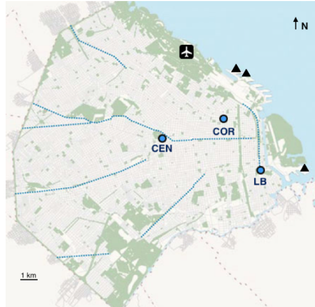
Figure 1: City of Buenos Aires (CBA) and location of the three air quality monitoring stations (CEN: Parque Centenario, COR: Córdoba, LB: La Boca). The locations of the AEP meteorological station at the Domestic Airport and three thermal power plants (triangles) are also indicated. Source: https://www.buenosaires.gob.ar/areas/med_ambiente/apra/calidad_amb/red_monitoreo/mapa.php?menu_id=32434 , accessed 09/29/2023
